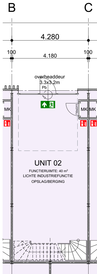
BEGANEGROUND (0.00)
